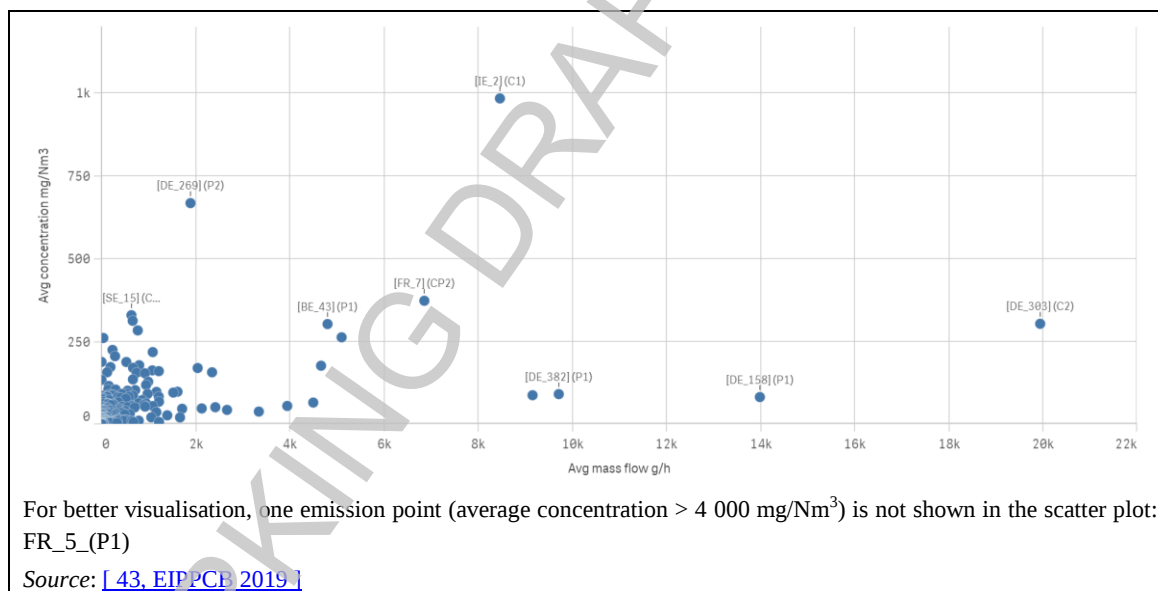
Figure 3.54: NO x concentration versus mass flow when thermal oxidation is used
