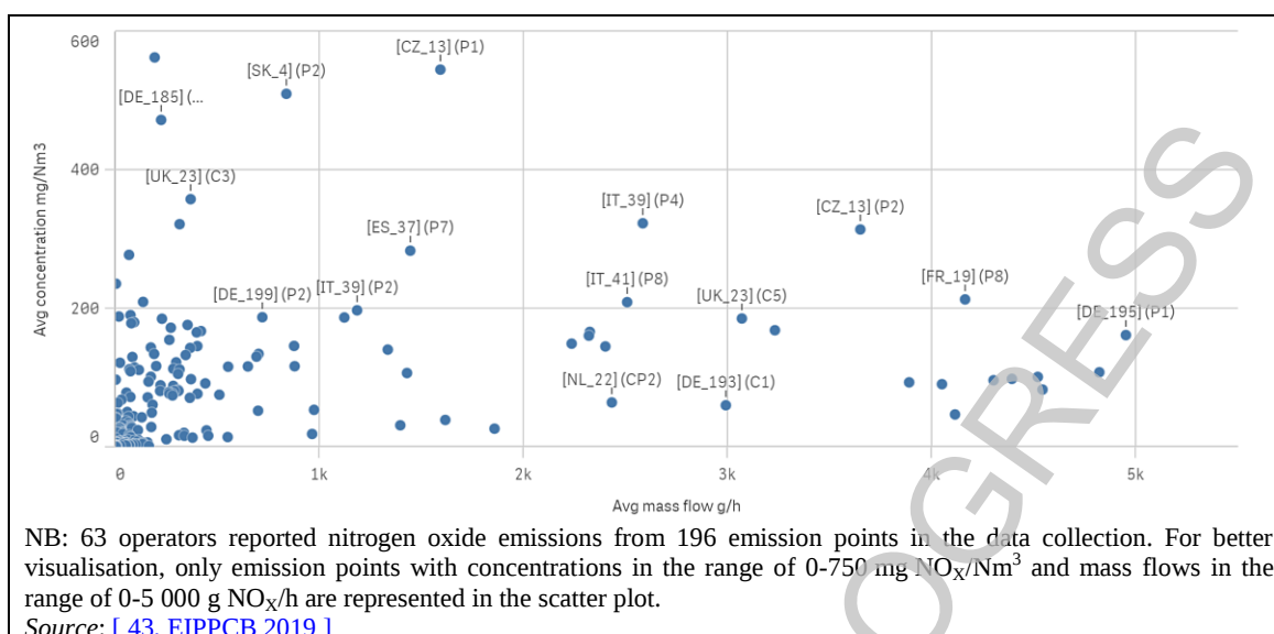
Figure 2.95: NO x emissions from chemical processes
