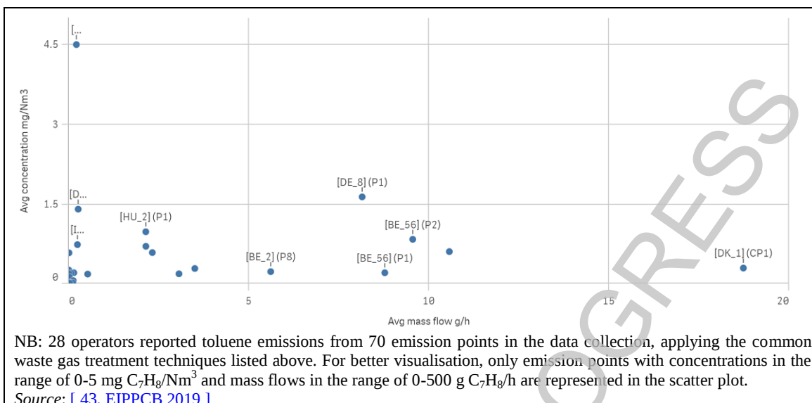
Figure 2.59: Toluene emissions after waste gas treatment
